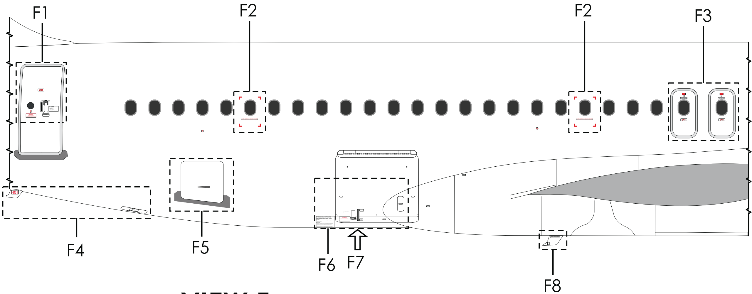
VIEW F RH FUSELAGE SECTION 46
