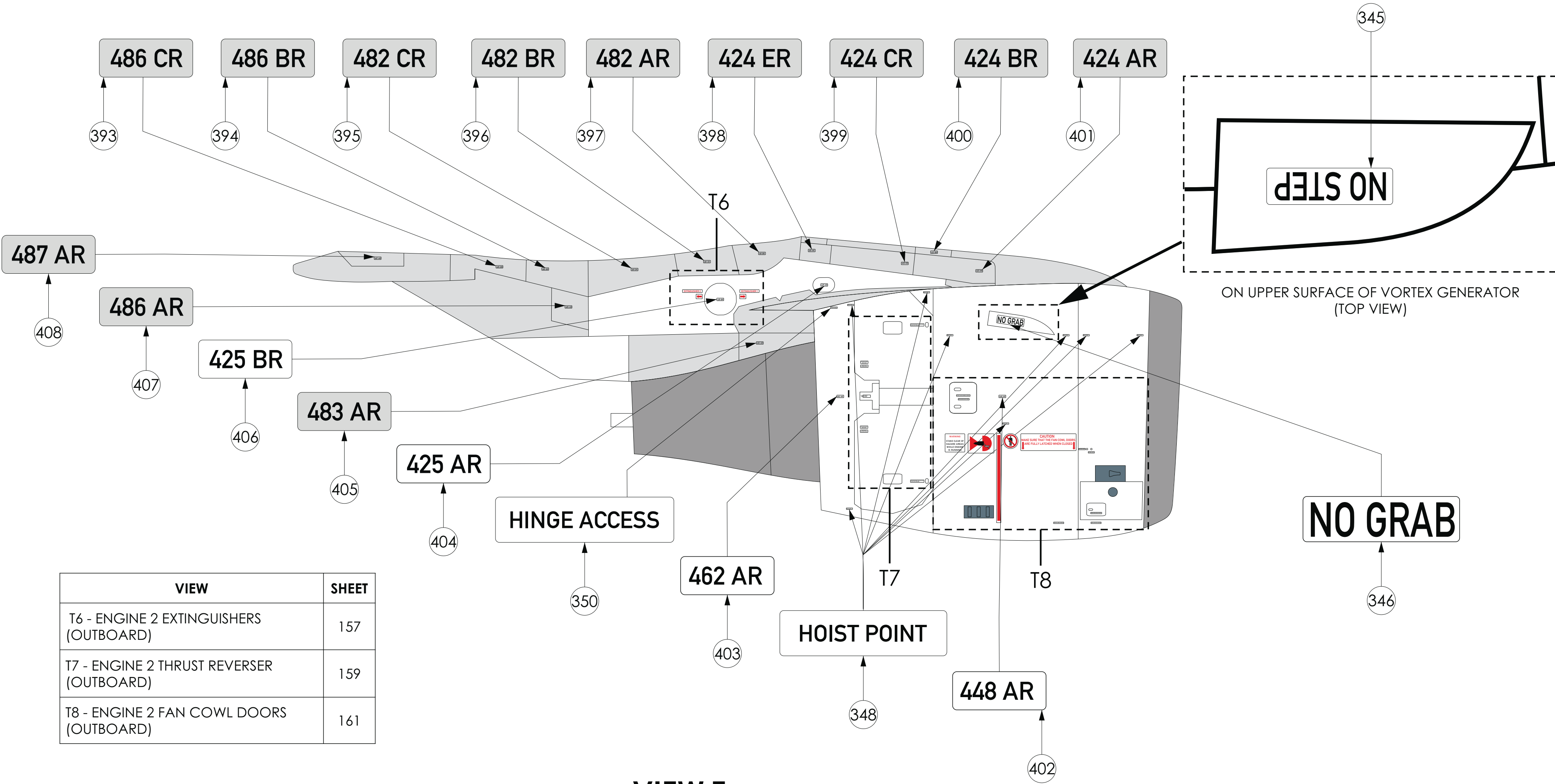
VIEW T ENGINE 2 (OUTBOARD)
