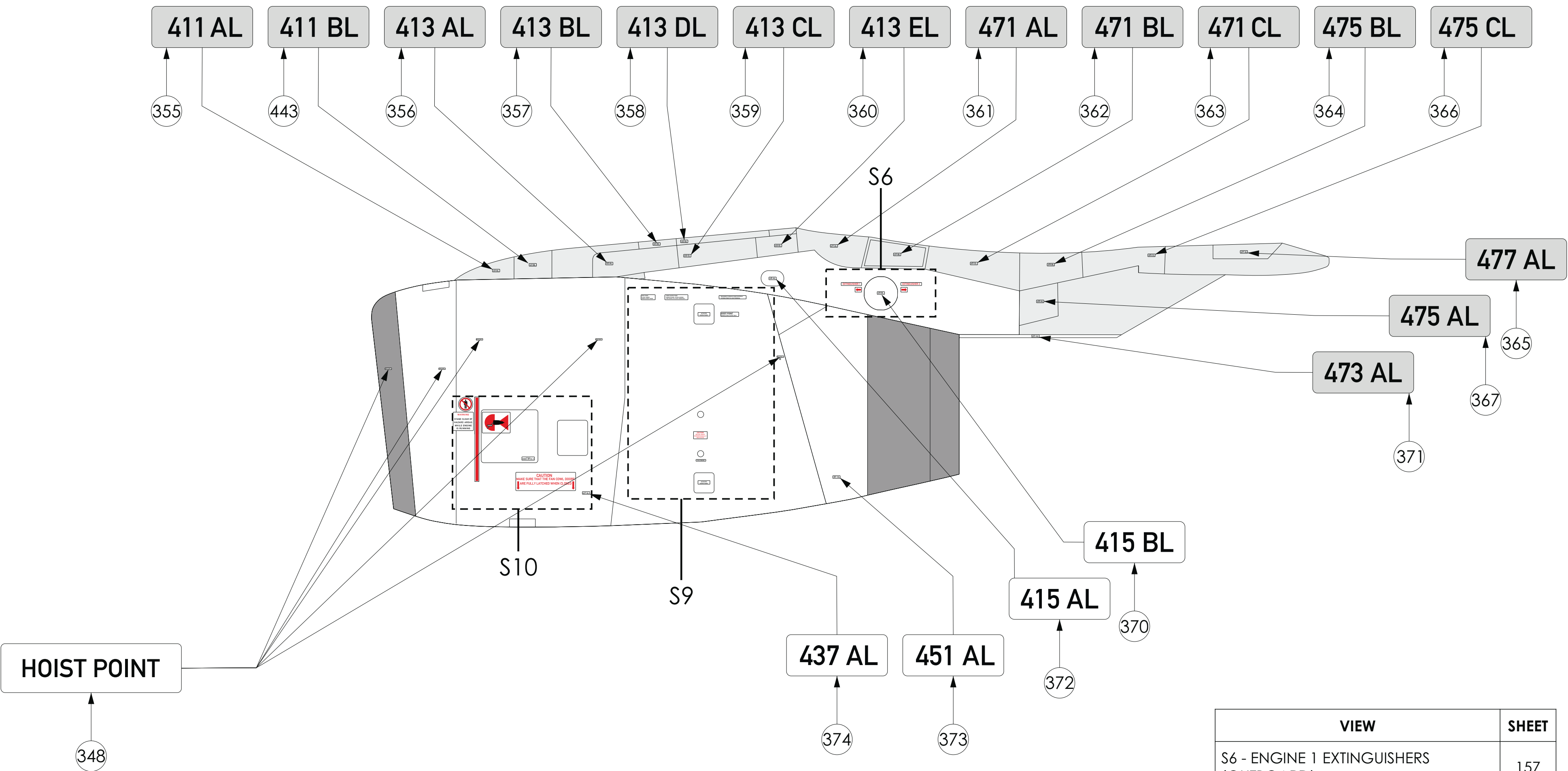
VIEW S ENGINE 1 (OUTBOARD)
